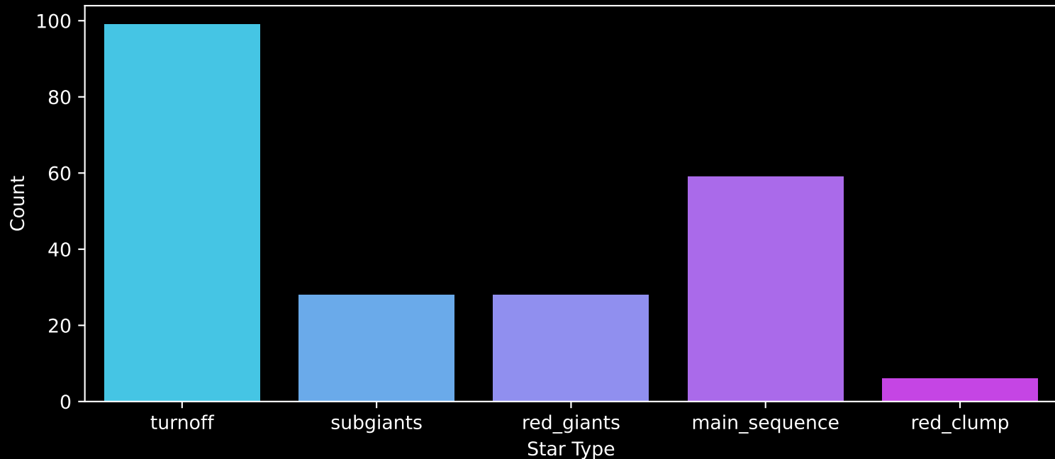
APOGEE DR17 Field: [ORIONOB1AB-A] Count plot of Star Type
