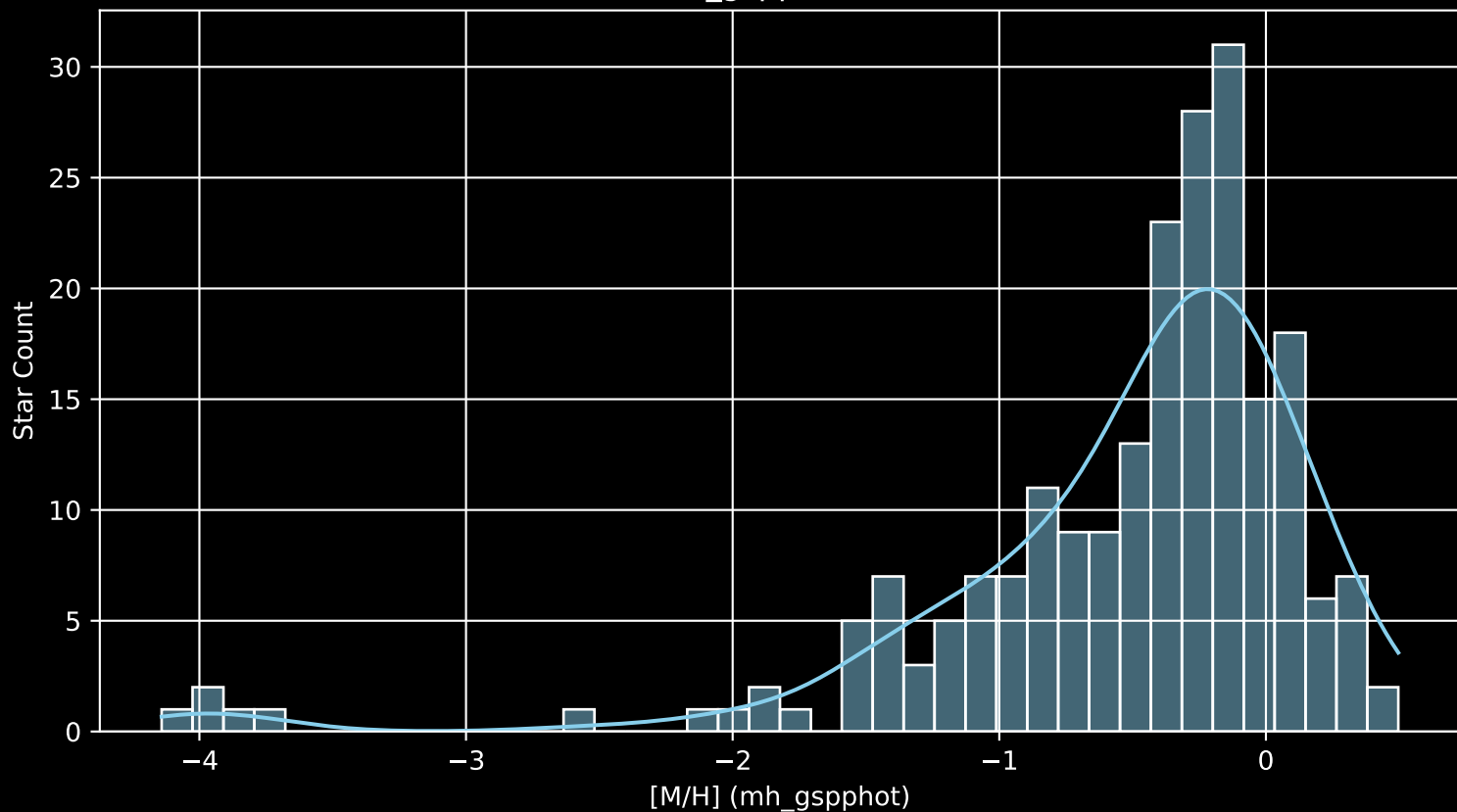
APOGEE DR17 Field: [ORIONOB1AB-A [M/H] (mh_gspphot) (n= 217)
