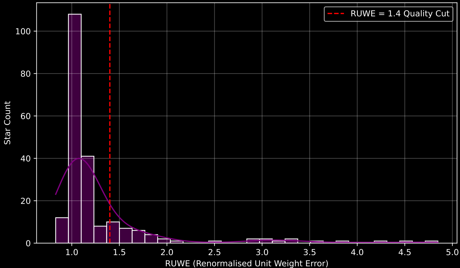
GAPOGEE DR17 Field [ORIONOB1AB-A] RUWE Distribution (n= 212)
