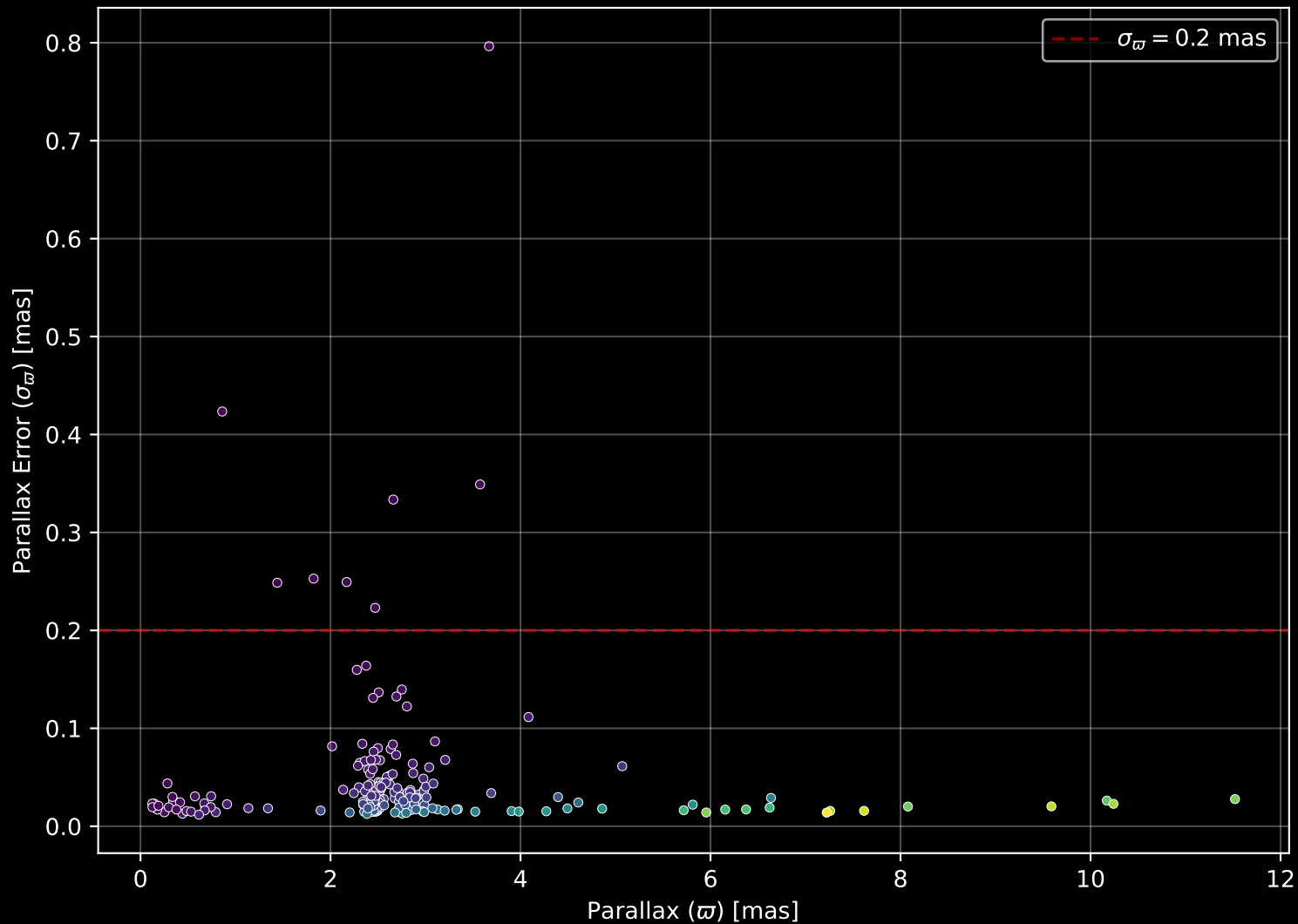
APOGEE DR17 Field: [ORIONOB1AB-A] Parallax Quality (n= 220)
