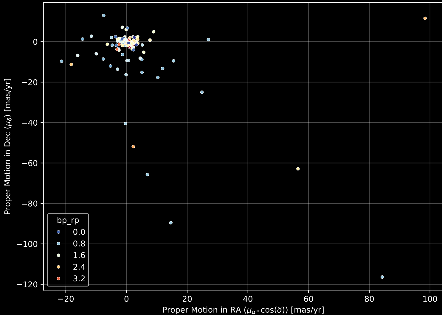
APOGEE DR17 Field: [ORIONOB1AB-A] Proper Motion Diagram (n= 220)
